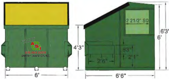
8 YARD SLANT SIDE DOOR
