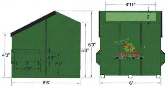
8 YARD FR. SLANT DOCK
