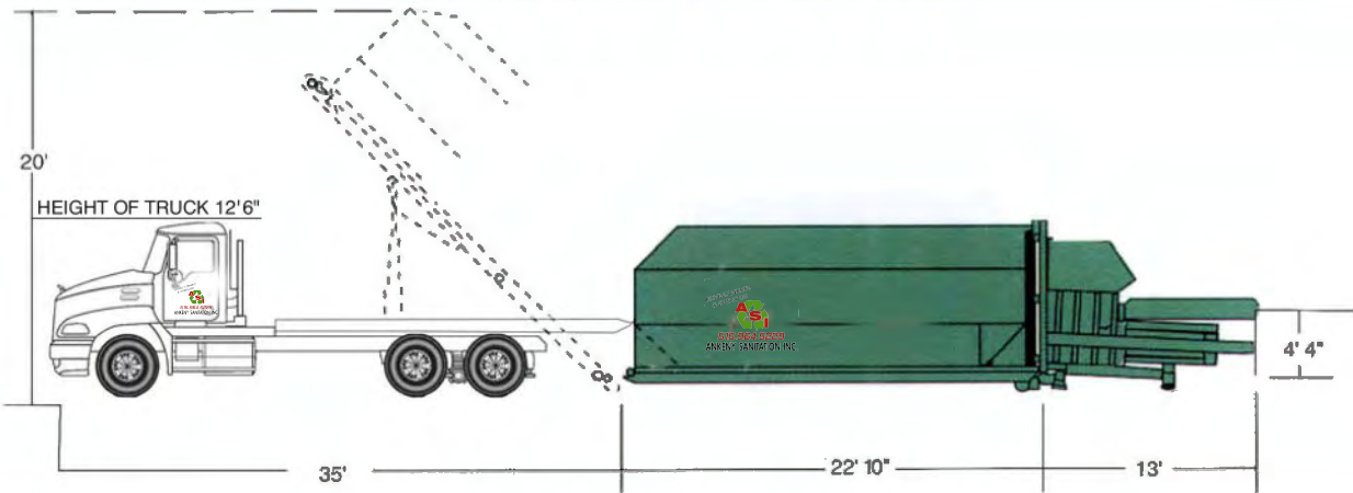
ROLL OFF VEHICLE CONFIGURATION
