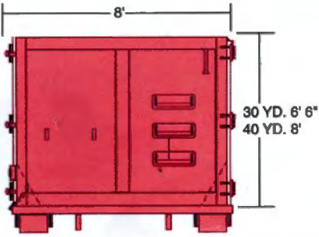
30 & 40 YARD OPEN TOP
