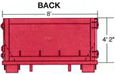
10 YARD OPEN TOP
