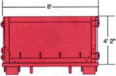
20 YARD OPEN TOP
